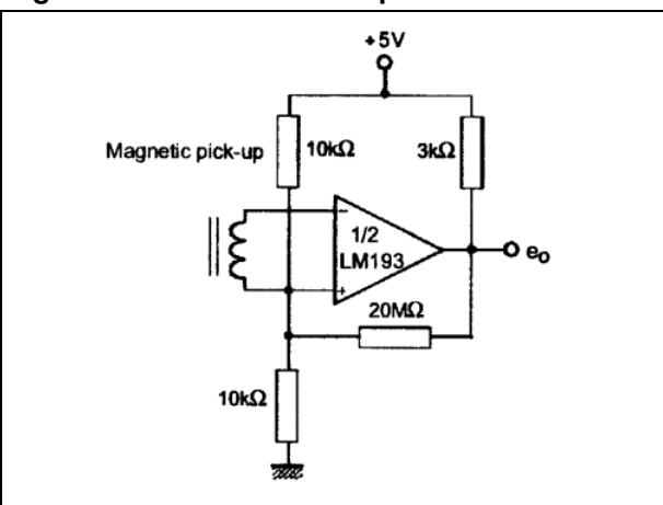
Figure 12. Transducer amplifier
