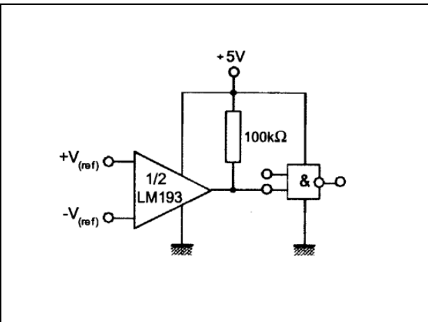
Figure 8. Driving CMOS
