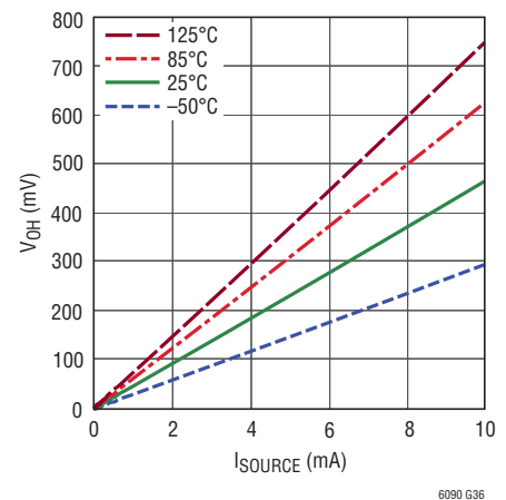
Output Voltage Swing High ( V_{\text{OH}} ) vs Load Current and Temperature
