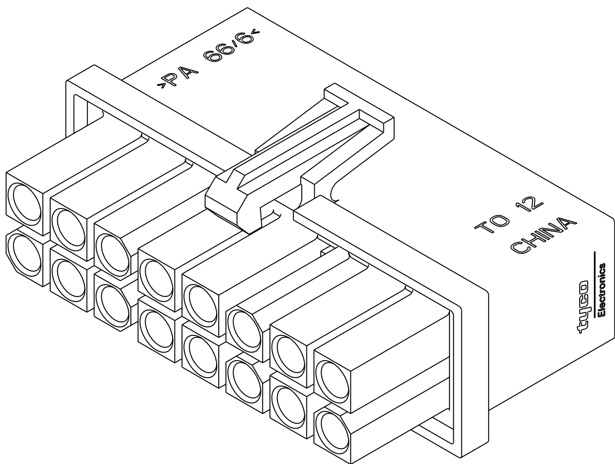
3 DIMENSIONAL MODEL SCALE 4:1
