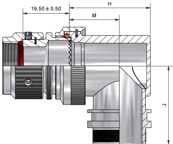
90° BACKSHELL - TYPE 2
