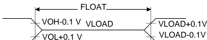
Figure 34. Float Waveforms
