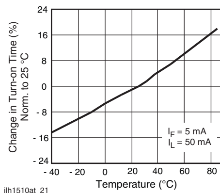
Fig. 22 - Turn-on Time vs. Temperature
