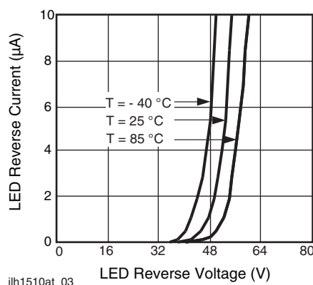
Fig. 4 - LED Reverse Current vs. LED Reverse Voltage
