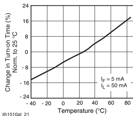
Fig. 22 - Turn-on Time vs. Temperature
