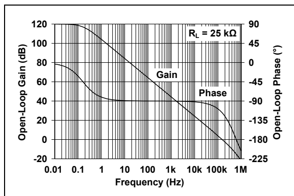
FIGURE 2-8: Open-Loop Gain and Phase vs. Frequency.
