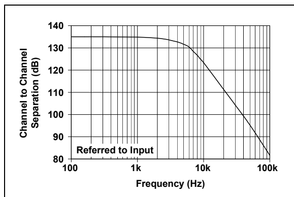
FIGURE 2-9: Channel-to-Channel Separation (MCP607 and MCP609 only).
