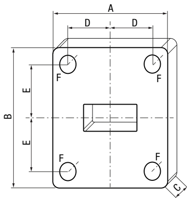
Rectangular Flanges
