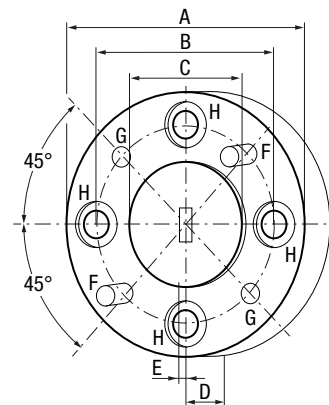
Circular Flanges
