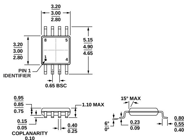
Figure 44. 8-Lead Mini Small Outline Package [MSOP] (RM-8) Dimensions show in millimeters
