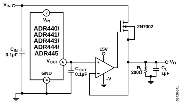
Figure 42. Boosted Output Reference
