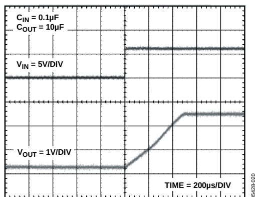
Figure 24. ADR441 Turn On Response
