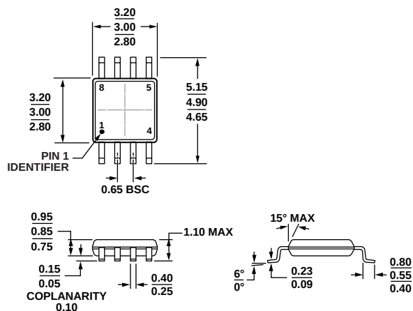
Figure 44. 8-Lead Mini Small Outline Package [MSOP] (RM-8) Dimensions show in millimeters
