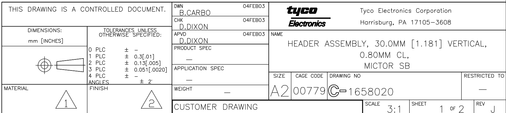
(BOTTOM VIEW) SCALE 2:1
