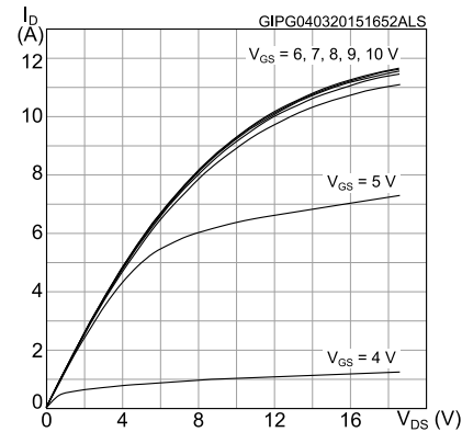
Figure 4: Output characteristics
