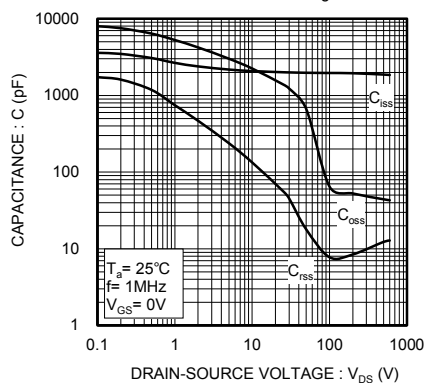
Fig.10 Typical Capacitance vs. Drain-Source Voltage
