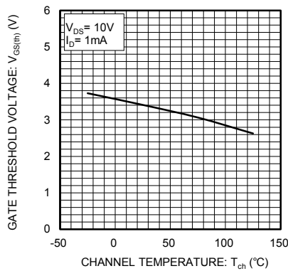
Fig.4 Gate Threshold Voltage vs. Channel Temperature
