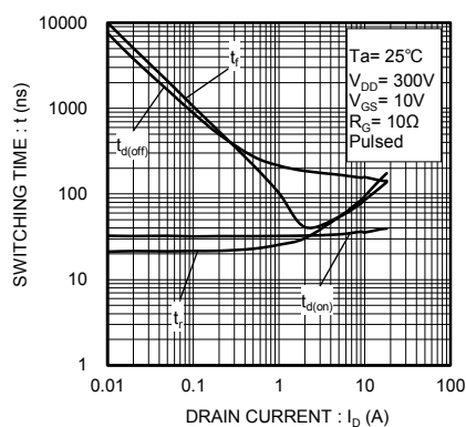
Fig.13 Switching Characteristics
