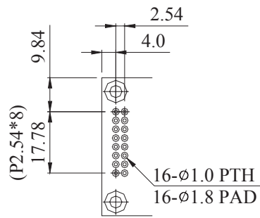
PIN DETAIL
