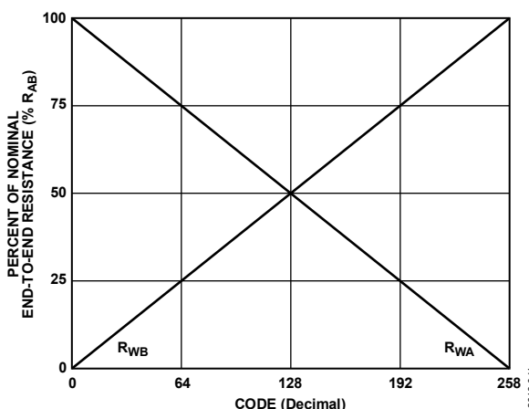
Figure 41. Symmetrical RDAC Operation
