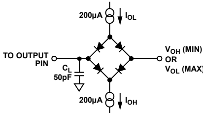
Figure 32. Load Circuit for Measuring V_{OH} and V_{OL}
