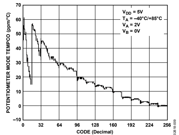
Figure 9. \Delta V_{WB}/\Delta T vs. Code; R_{AB} = 10\text{ k}\Omega, V_{DD} = 5\text{ V}
