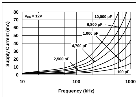
FIGURE 2-17: Supply Current vs. Frequency.
