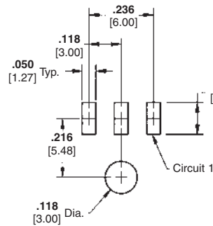
Recommended PC Board Layout * 3 Position
