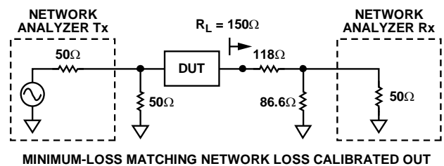
Figure 15. Basic Test Circuit for Swept Frequency Measurements
