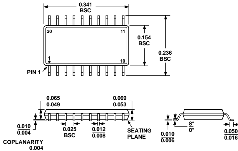
Figure 21. 20-Lead Shrink Small Outline Package [QSOP] (RQ-20) Dimensions shown in inches
