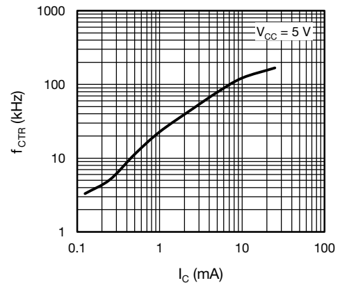
Fig. 15 - Cut-off Frequency (-3 dB) vs. Collector Current
