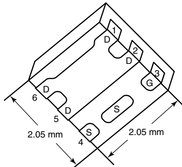
PowerPAK SC-70-6L-Single
