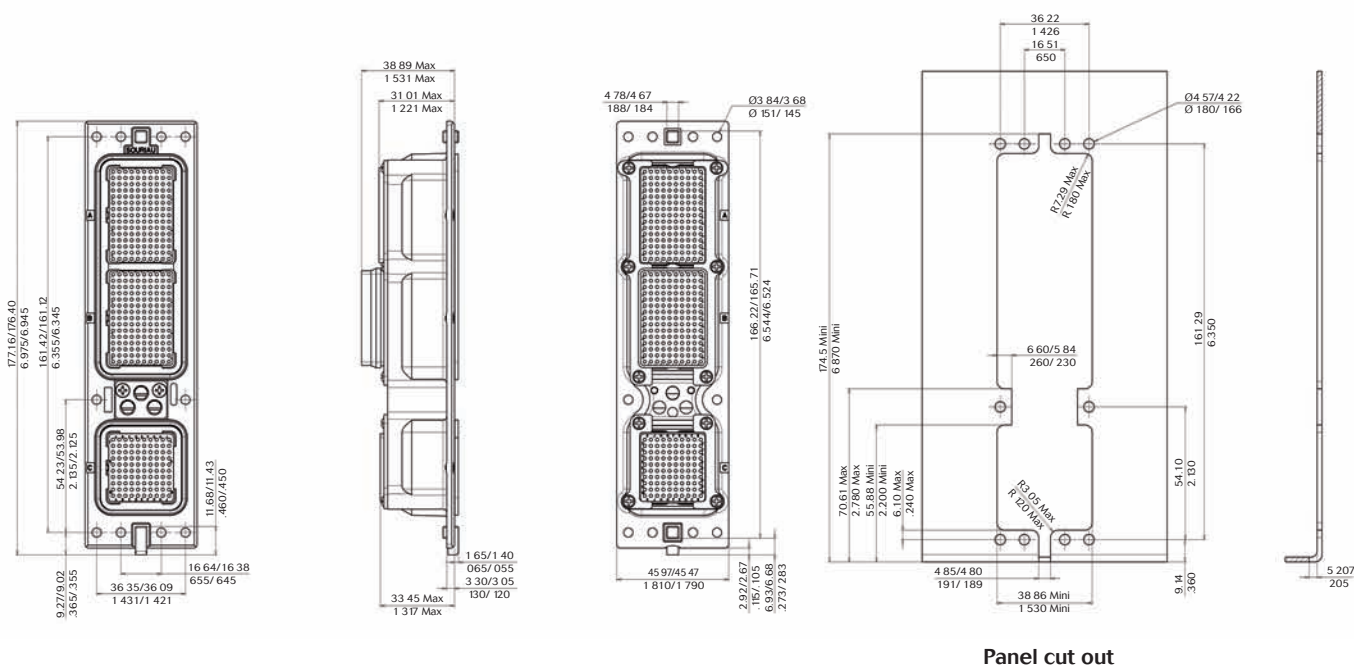
Shell Size 2 - Equipment Receptacle (mm/inch)
