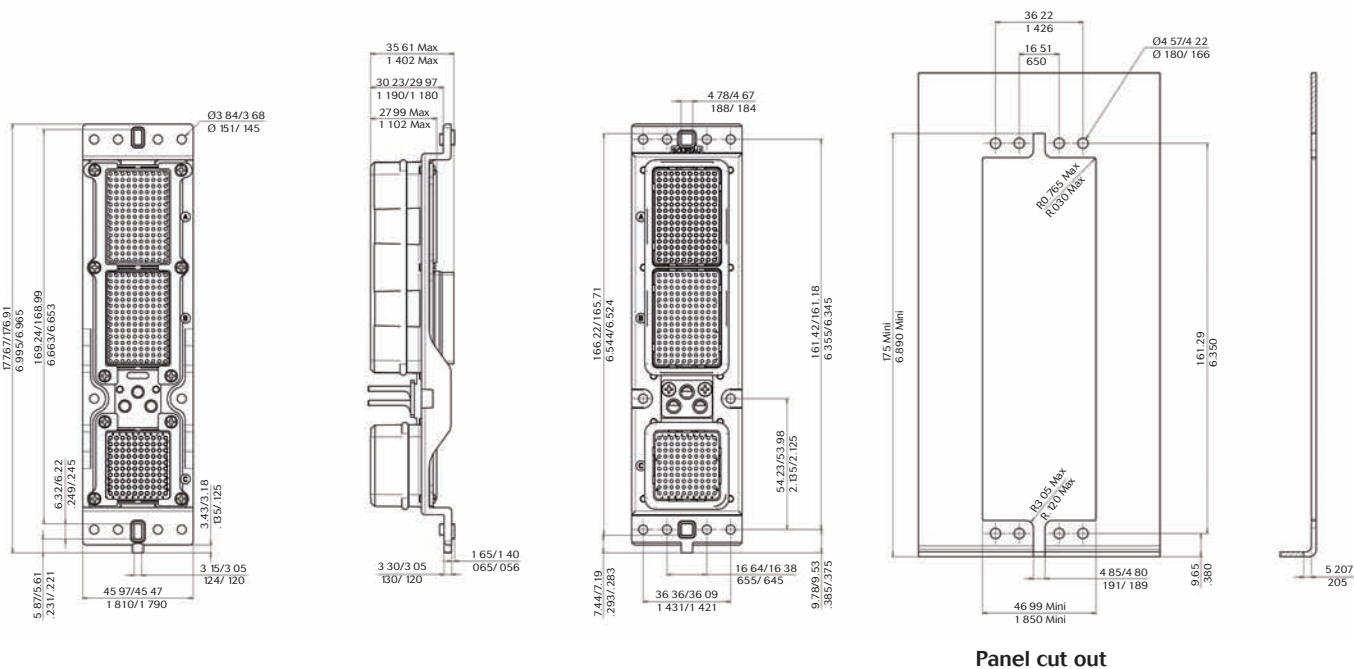
Shell Size 2 - Rack Plug (mm/inch)
