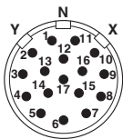
Contact chamber numbering (view of plug-in side), pin counter direction
