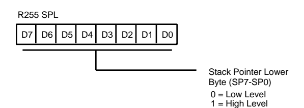
Figure 66. Stack Pointer (F FH : Read/Write)
