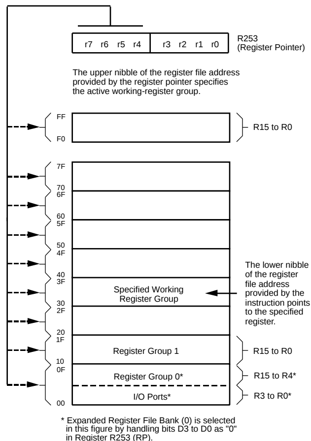
Figure 18. Register Pointer
