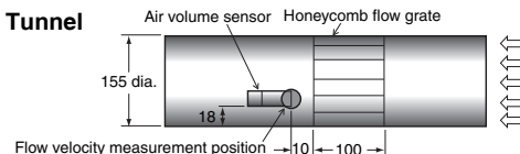
Figure 2: Wind Tunnel
