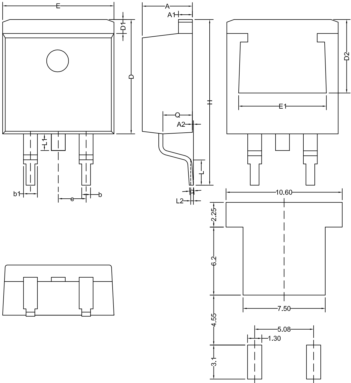
Recommended Footprint
