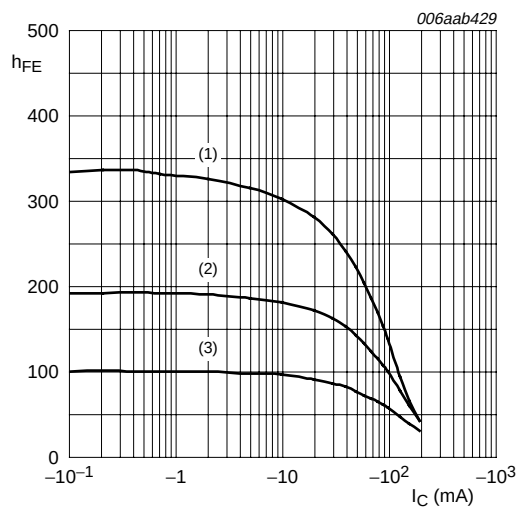
V_{CE} = -5 V (1) T_{amb} = 150 °C (2) T_{amb} = 25 °C (3) T_{amb} = -55 °C
