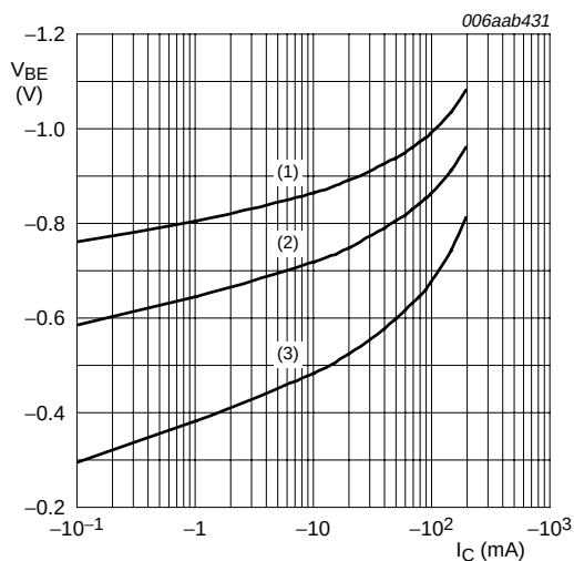
V_{CE} = -5 V (1) T_{amb} = -55 °C (2) T_{amb} = 25 °C (3) T_{amb} = 150 °C
