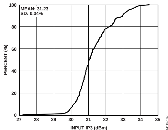
Figure 32. Input IP3 Distribution
