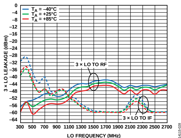
Figure 28. 3 \times LO Leakage vs. LO Frequency over Three Temperatures ( 3 \times LO to RF and 3 \times LO to IF)
