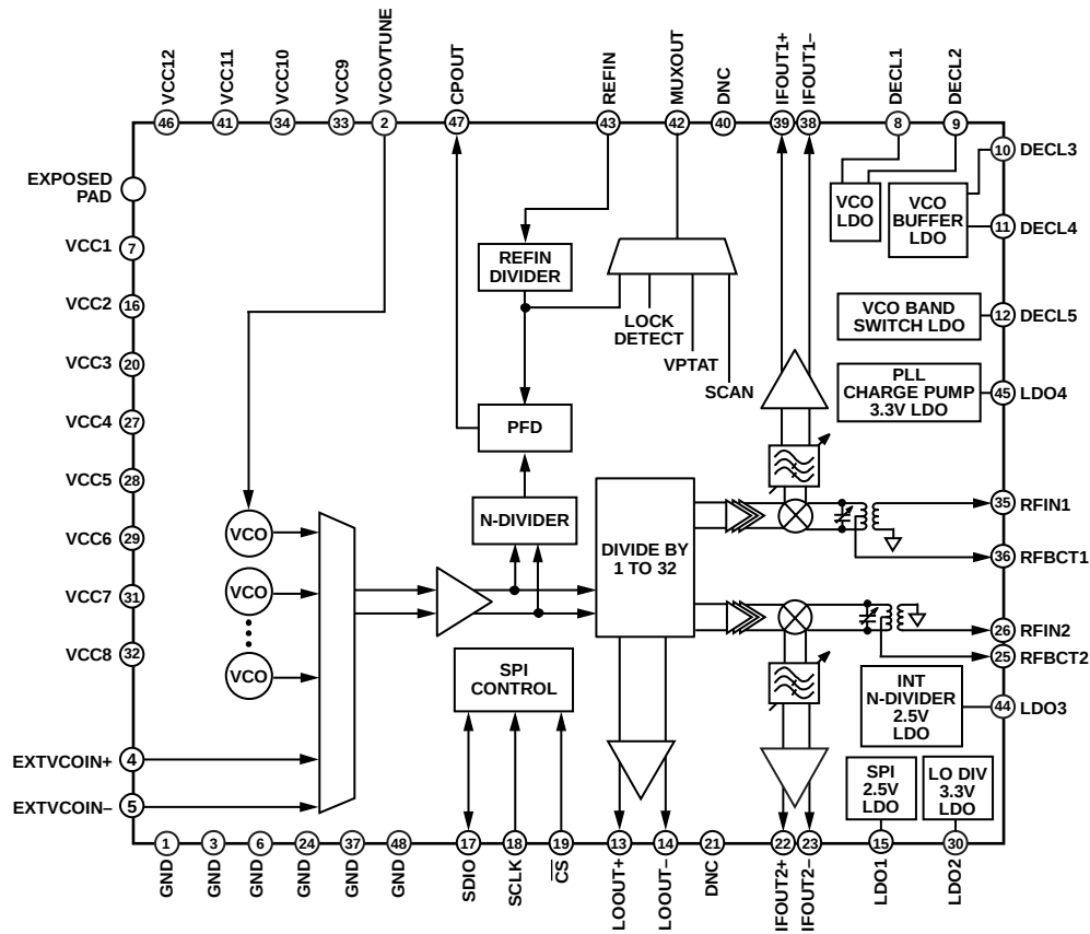
Figure 110. Simplified Schematic
