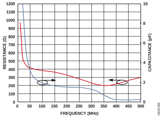
Figure 34. IF Output Impedance (R Parallel C Equivalent)
