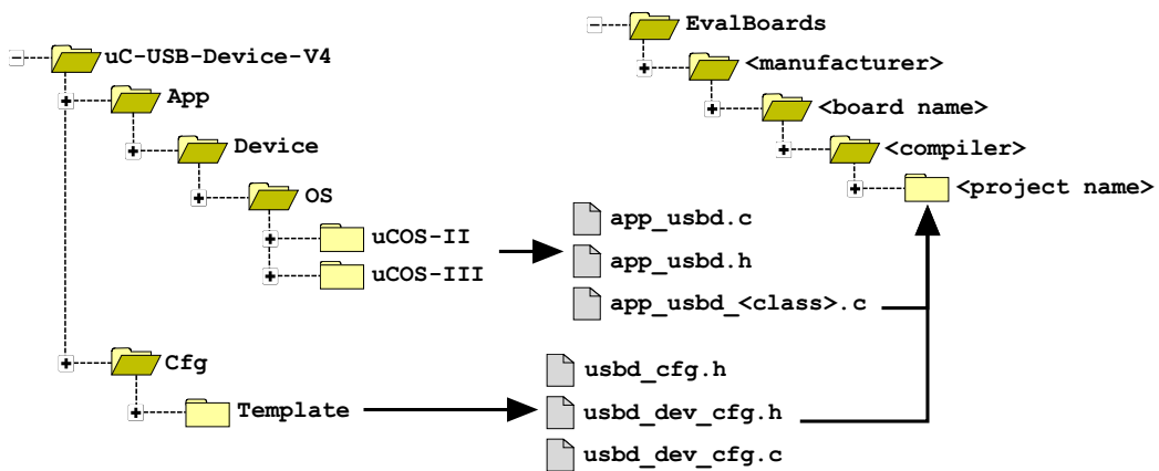
Figure 2-2 Copying Template Files.
