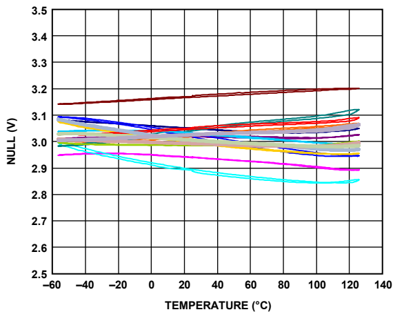
Figure 6. Null Output over Temperature, 16 Parts in Sockets
