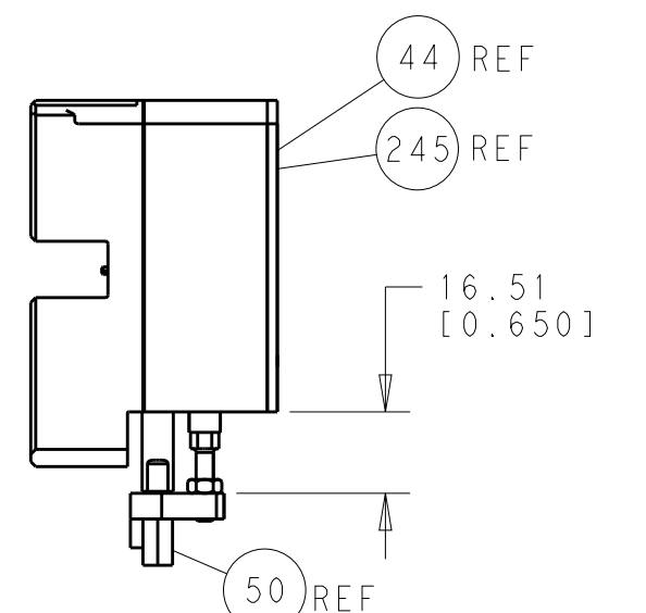
HOLDDOWN SET-UP
