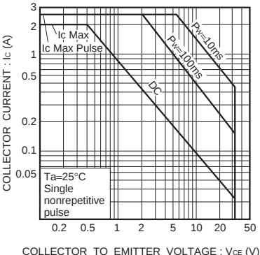
Fig.9 Safe operating area (2SD1862)
