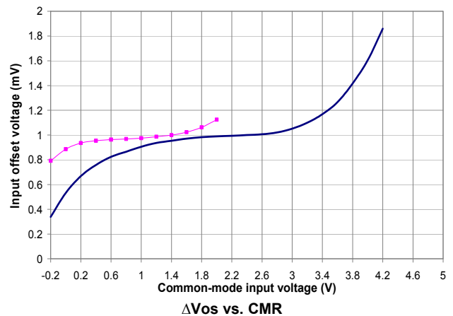
\Delta V_{os} vs. CMR
