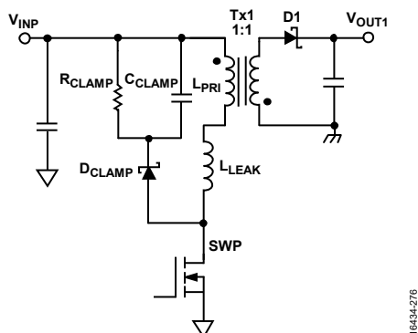
Figure 72. Resistor, Capacitor, Diode Clamp
