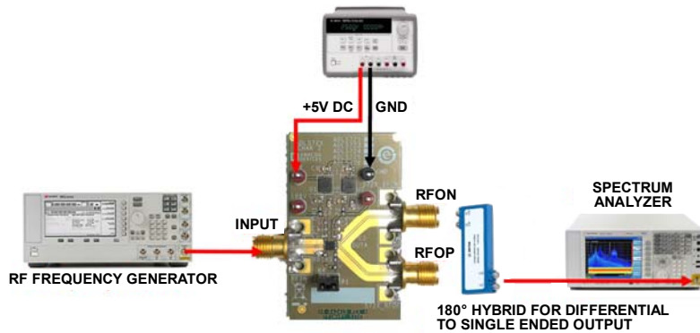
Figure 19. ADL5724-EVALZ Lab Bench Setup
