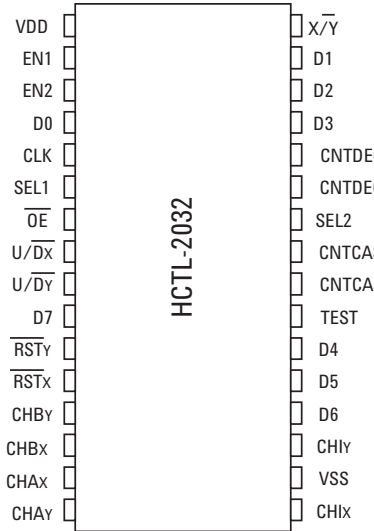
PINOUT A
