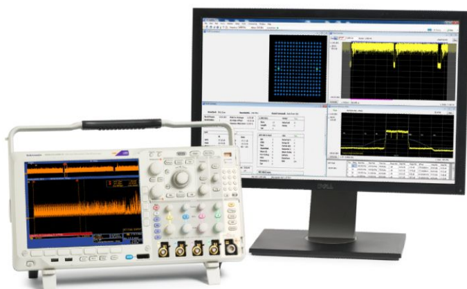
MDO4000C paired with SignalVu-PC to analyze 802.11ac modulation.
