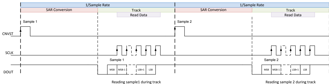
Figure 3. Conversion Frame, SAR Conversion, Track and Read Operation
