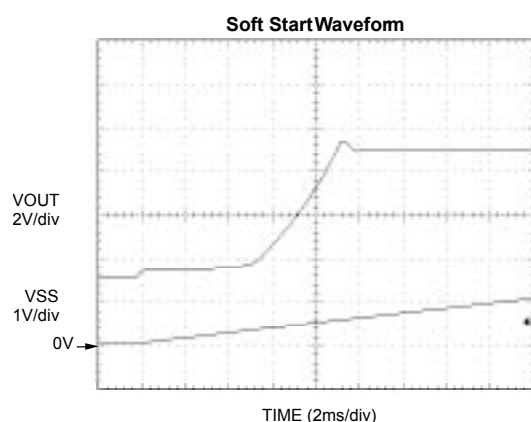
Figure 10 Soft Start
