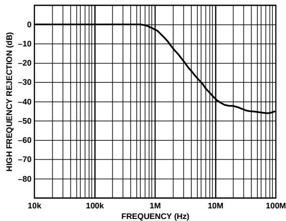
Figure 34. Frequency Response of Second-Order Butterworth Filter
