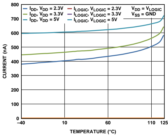
Figure 16. Supply Current vs. Temperature
