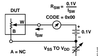
Figure 37. Power Supply Sensitivity and Power Supply Rejection Ratio (PSS and PSRR)
