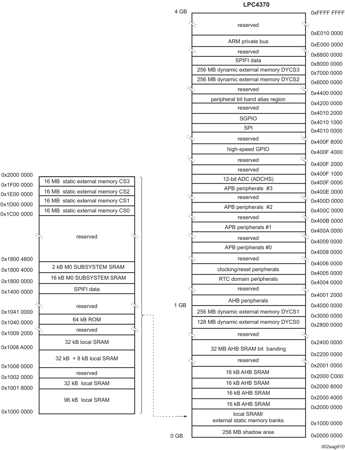
Fig 5. LPC4370 Memory mapping (overview)
