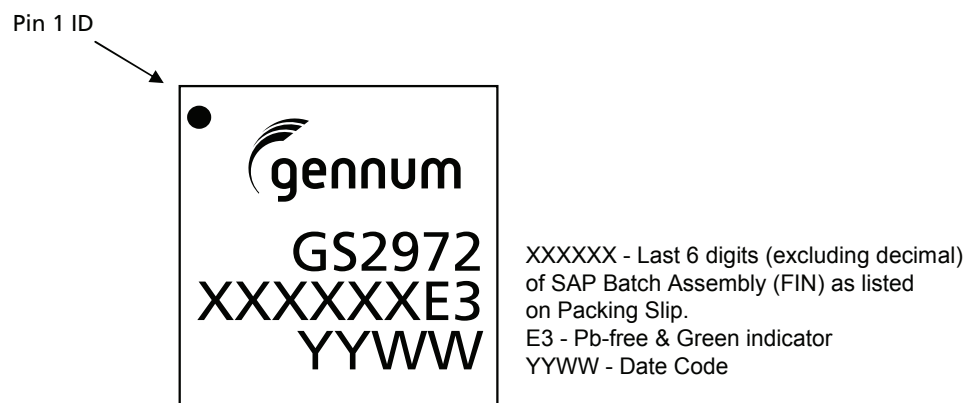
Figure 7-2: Marking Diagram
