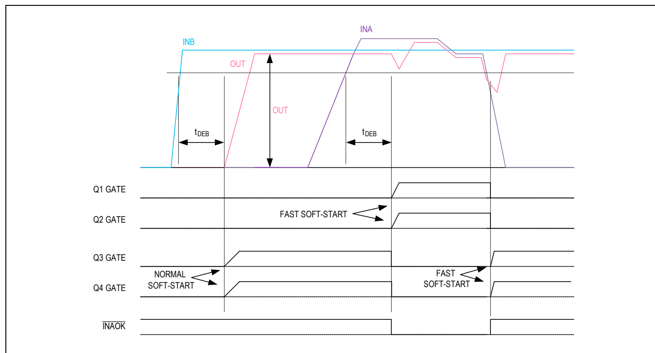
Figure 2. Automatic Switch Operation, PCON = 1
