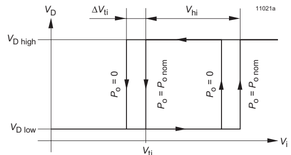
Fig. 37 Definition of V_{ti} , \Delta V_{ti} and \Delta V_{hi} (JFET output)
